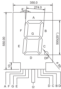
BL-SE2000DP
