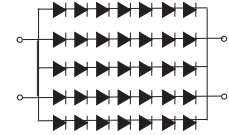
BL-SE800EA
