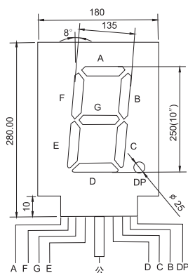
BL-SE1000EA
