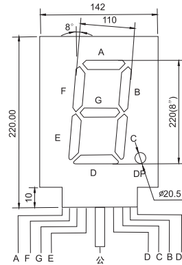
BL-SE800EA
