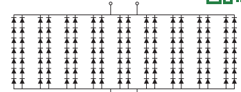
BL-SE2000DP
